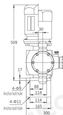
GBS series size chart (including base)
